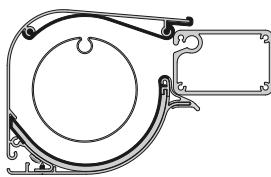
End cap of the box in the retracted condition
